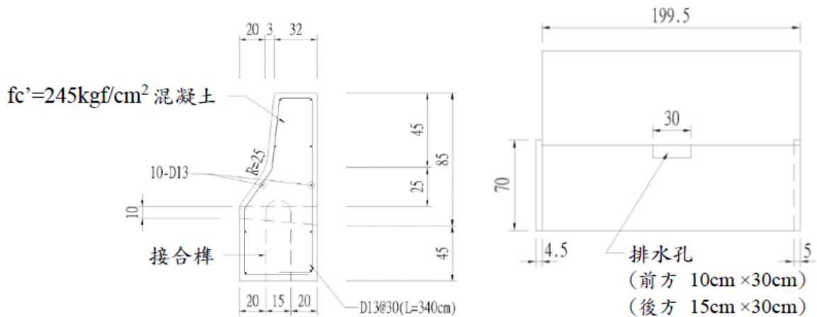
斷面及配筋
